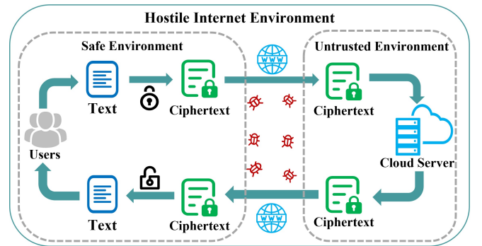
Fig. 1: FHE in Service-oriented Scenarios
